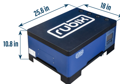
RGS51100 MODEL WITH BASE AND LID
