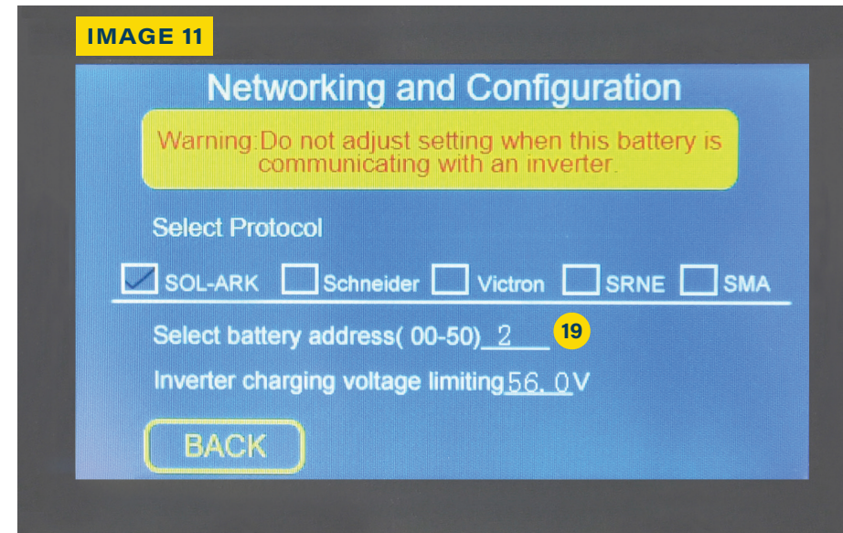
19 SELECT BATTERY ADDRESS.
